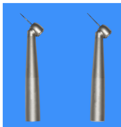
图6 45°仰角冲击式气动手机及外科车针 Fig.6 45-degree inclined impact air handpiece and surgical burs.
